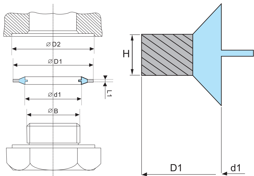
Bonded Seal 804 Type Size List
